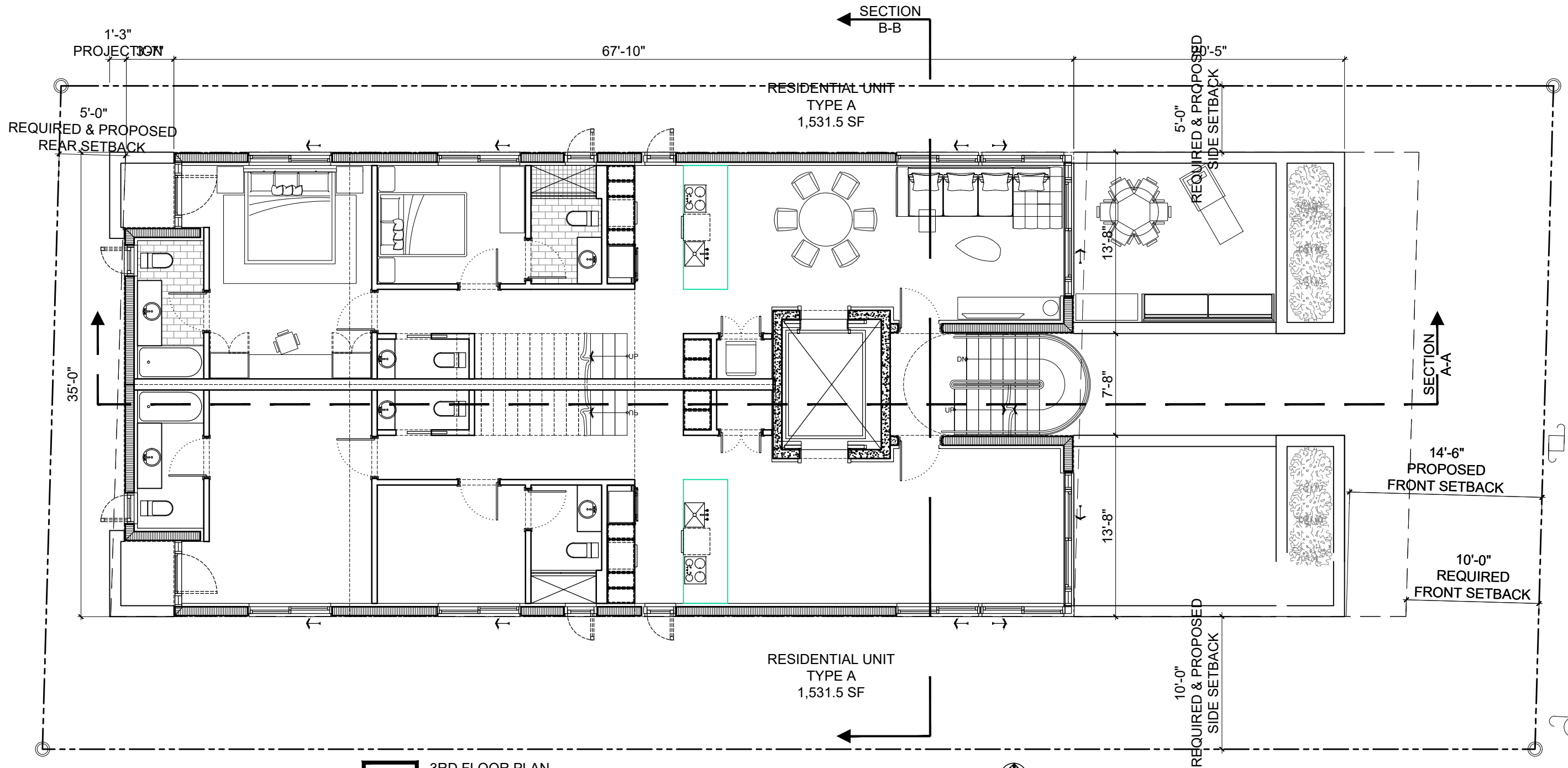
1 3RD FLOOR PLAN SCALE: 1/8" = 1'-0"
